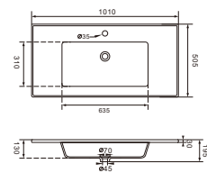
938-100 Cabinet Basin 1010x505x195mm
