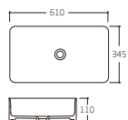
K-M6260-60B Wash Basin 610x345x110mm
