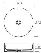
K-6425 Wash Basin 370x370x130mm
