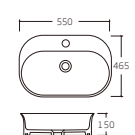
K-6337 Wash Basin 550x465x150mm
