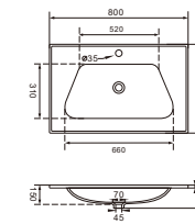
910-80 Cabinet Basin 800x500x200mm
