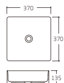
K-6324-37 Wash Basin 370x370x135mm
