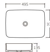
K-6360 Wash Basin 495x375x135mm
