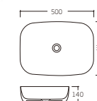
K-6210 Wash Basin 500x380x140mm
