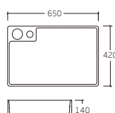
K-6462-6542L Wash Basin 650x420x140mm
