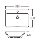
K-6335 Wash Basin 555x420x125mm
