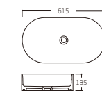
K-6265 Wash Basin 615x415x135mm
