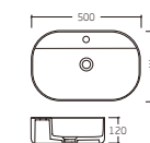
K-6243 Wash Basin 500x380x120mm
