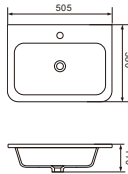
911-50/911-61 Cabinet Basin 911-50: 505x380x170mm 911-61: 600x455x170mm
