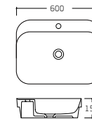
K-6420-60 Wash Basin 600x420x155mm
