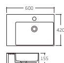
K-6452R Wash Basin 600x420x155mm
