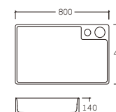
K-6462-8042R Wash Basin 800x420x140mm
