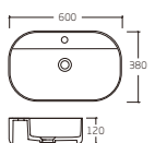
K-6298 Wash Basin 600x380x120mm
