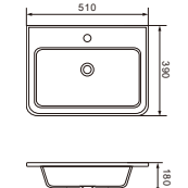
909-51/909-64 Cabinet Basin 909-51: 510x390x180mm 909-64: 640x480x205mm
