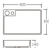
K-6462-6035L Wash Basin 600x350x140mm
