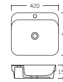
K-6420-42 Wash Basin 420x420x155mm
