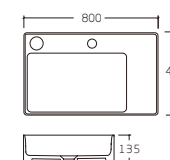
K-6463-80 Wash Basin 800x475x135mm
