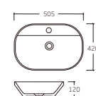
K-6332 Wash Basin 505x420x120mm
