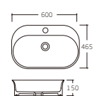
K-6338 Wash Basin 600x465x150mm
