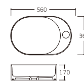
K-6464-46/K-6464-56 Wash Basin 6464-46: 460x320x170mm 6464-56: 560x360x170mm
