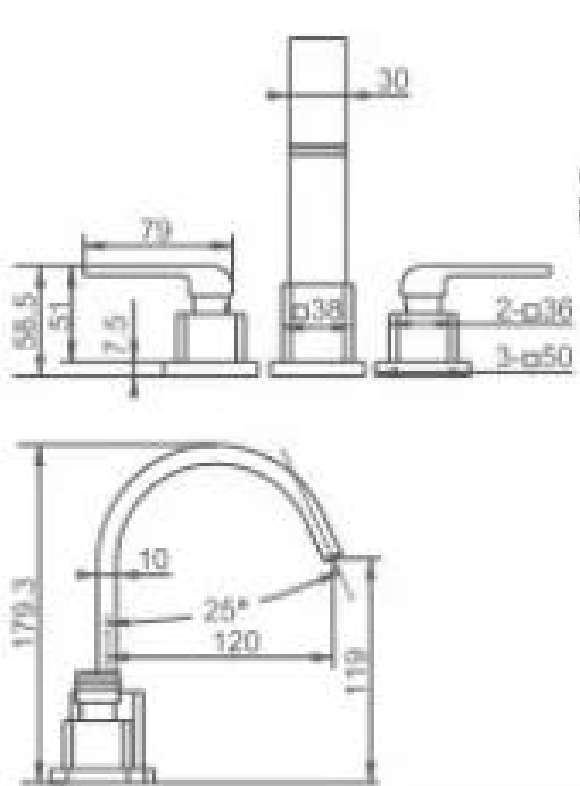
25008 双把分体面盆龙头 Single handle basin faucet 主体材质：铜 /Material: Brass
