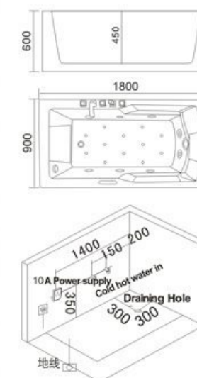
Model: H-003B SIZE: 1500x800x600mm 1700x830x600mm 1800x900x600mm 左右裙 Left/Right Skirt
