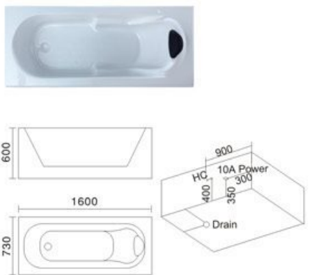
Model: H-071 SIZE: 1500x700x600mm 1600x730x600mm 1700x730x600mm 左右裙 Left/Right Skirt
