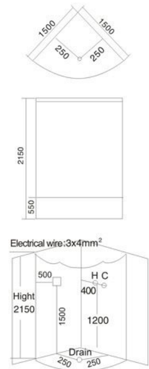
Model: A-083 SIZE: 1500x1500x2150mm
