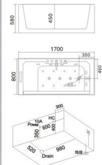
Model: H-1702 SIZE: 1700x800x580mm
