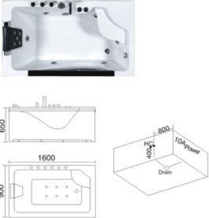
Model: H-1690 SIZE: 1600x900x650mm 左右裙 Left/Right Skirt
