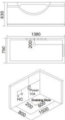
Model: H-1687 SIZE: 1380x750x630mm 1500x800x630mm 左右裙 Left/Right Skirt
