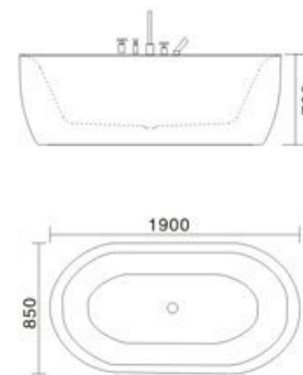
Model: H-006 SIZE: 1900x850x730mm
