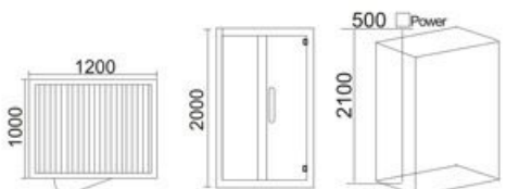
LN-1062 铁杉木 Hemlock 1200x1000x2000mm 非标订造 Non-standard manufactured 可做桑拿房、光波房、频谱房 Saund Room、Far-Infrsred Steam Room、 Spectrum Room
