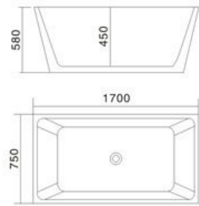
Model: H-7002 SIZE: 1300x700x580mm 1400x700x580mm 1500x700x580mm 1600x700x580mm 1700x700x580mm 1500x750x580mm 1600x750x580mm 1700x750x580mm
