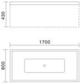
Model: H-7002D SIZE: 1500x750x430mm 1600x750x430mm 1700x800x430mm
