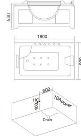
Model: H-1815 SIZE: 1800x900x630mm 左右裙 Left/Right Skirt
