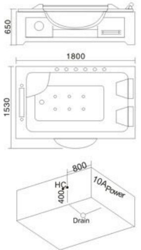
Model: H-1816 SIZE: 1800x1530x650mm 左右裙 Left/Right Skirt
