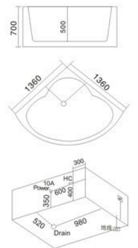
Model: H-1688 SIZE: 1360x1360x700mm
