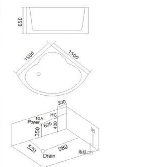
Model: H-1512 SIZE: 1500x1500x650mm
