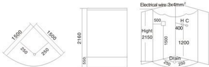
Model: A-082 SIZE: 1360x1360x2160mm 1500x1500x2160mm 1650x1650x2160mm
