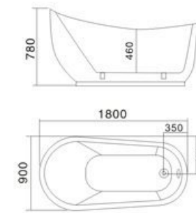
Model: H-7061 SIZE: 1800x900x780mm 1700x800x750mm 1600x750x800mm 1500x750x800mm
