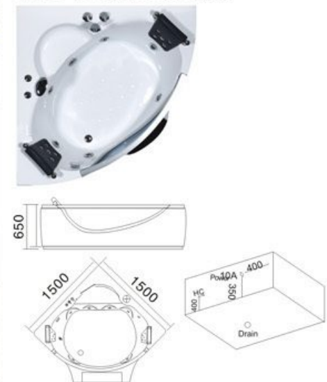
Model: H-1512A SIZE: 1500x1500x650mm
