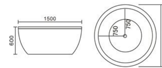
Model: H-7035 SIZE: 1500x1500x600mm
