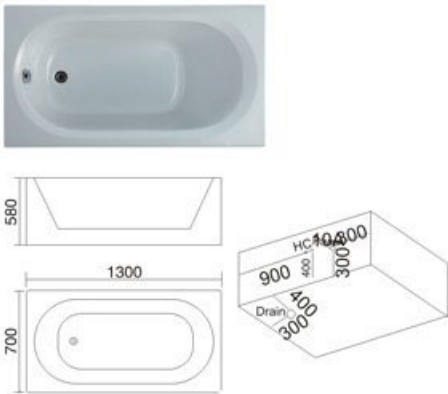
Model: H-070 SIZE: 1200x700x580mm 1300x700x580mm 1400x700x580mm 1500x700x580mm 1600x700x580mm 左右裙 Left/Right Skirt
