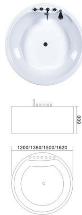
Model: H-7032 SIZE: 1200x1200x600mm 1380x1380x600mm 1500x1500x600mm 1620x1620x600mm
