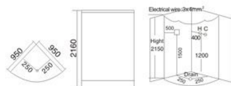
Model: A-002 SIZE: 950x950x2160mm
