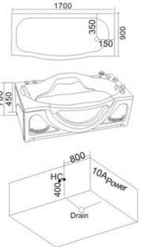
Model: H-1790 SIZE: 1700x900x700mm
