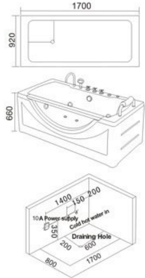
Model: H-1519 SIZE: 1700x920x660mm
