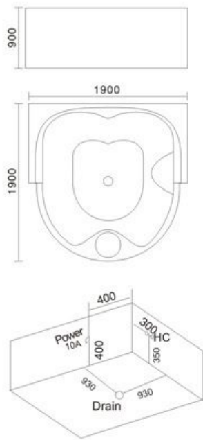
Model: H-5613 SIZE: 1900x1900x900mm
