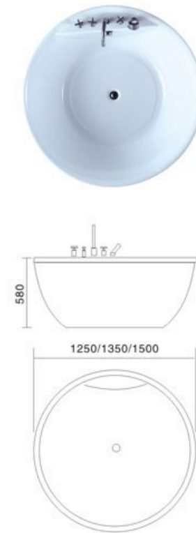
Model: H-7038 SIZE: 1250x1250x580mm 1350x1350x580mm 1500x1500x580mm
