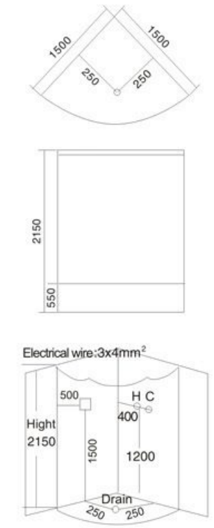
Model: A-090 SIZE: 1500x1500x2150mm
