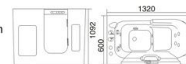
Model: H-5630 SIZE: 1320x600x1092mm
