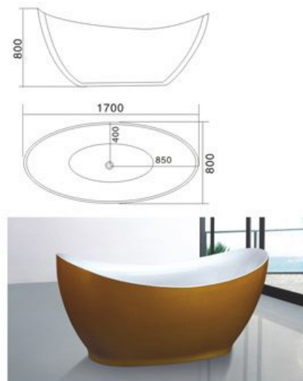
Model: H-7020 SIZE: 1700x800x800mm
