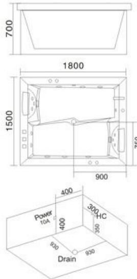
Model: H-1815 SIZE: 1800x1500x700mm
