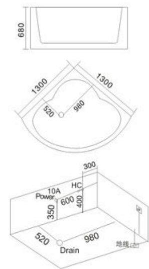
Model: H-1313 SIZE: 1300x1300x680mm
