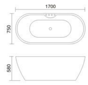
Model: H-7110 SIZE: 1700x750x580mm
