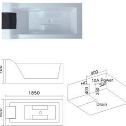
Model: H-1883 SIZE: 1850x850x700mm 左右裙 Left/Right Skirt
