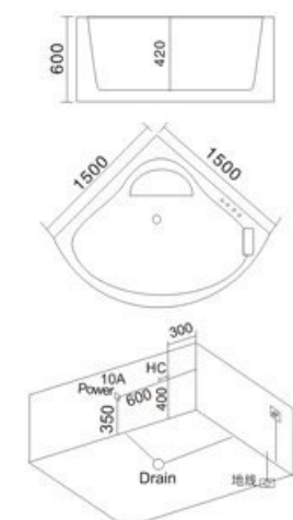
Model: H-055B SIZE: 1500x1500x600mm
