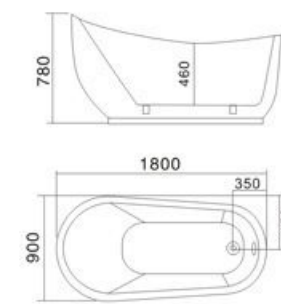
Model: H-7062 SIZE: 1800x900x780mm 1700x800x750mm 1600x750x800mm 1500x750x800mm
