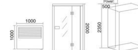
LN-1023 铁杉木 Hemlock 1000x1000x2000mm 非标订造 Non-standard manufactured 可做桑拿房、光波房、频谱房 Saund Room、Far-Infrsred Steam Room、 Spectrum Room
