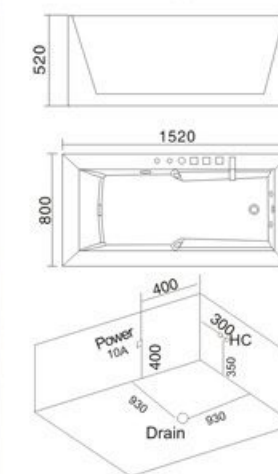
Model: H-058 SIZE: 1520x800x520mm 1710x800x520mm 左右裙 Left/Right Skirt
