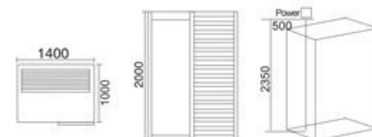
LN-1003 铁杉木 Hemlock 1400x1000x2000mm 非标订造 Non-standard manufactured 可做桑拿房、光波房、频谱房 Saund Room、Far-Infrsred Steam Room、 Spectrum Room
