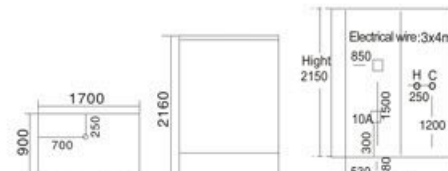
Model: A-024 SIZE: 1700x900x2160mm
