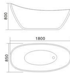
Model: H-7026 SIZE: 1800x850x800mm
