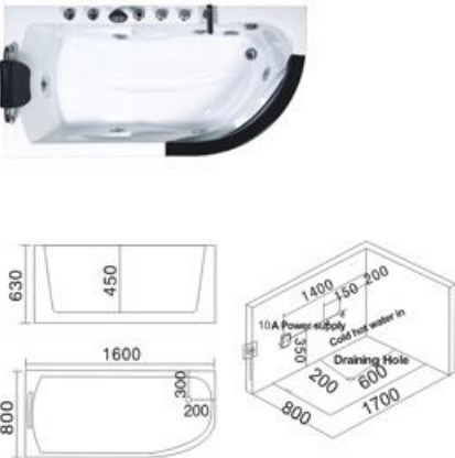
Model: H-1689 SIZE: 1500x800x630mm 1600x800x630mm 1700x800x630mm 左右裙 Left/Right Skirt
