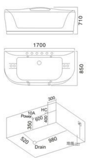
Model: H-010 SIZE: 1700x850x710mm
