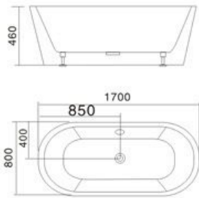
Model: H-13 SIZE: 1400x700x460mm 1500x750x460mm 1600x750x460mm 1600x800x460mm 1700x800x460mm 1780x800x460mm
