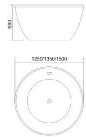
Model: H-7037 SIZE: 1250x1250x580mm 1350x1350x580mm 1500x1500x580mm
