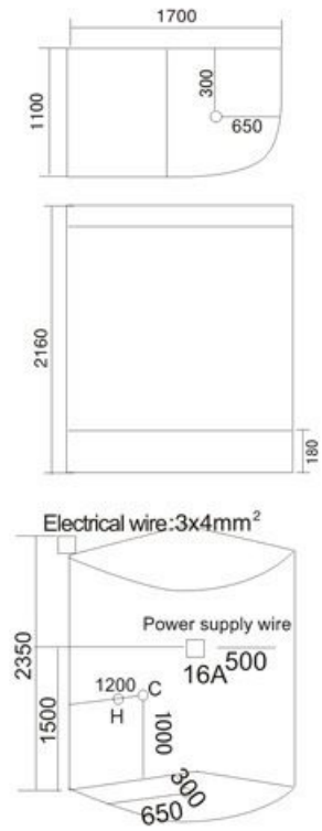
Model: LN-1711A SIZE: 1700x1100x2160mm 1600x1100x2160mm 左右 Left/Right
