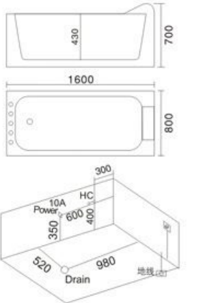
Model: H-1022 SIZE: 1600x800x700mm 1700x800x700mm 左右裙 Left/Right Skirt
