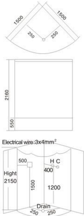
Model: A-082B SIZE: 1500x1500x2160mm
