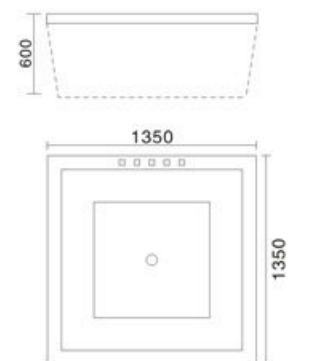
Model: H-029A SIZE: 1350x1350x600mm 1650x1650x600mm
