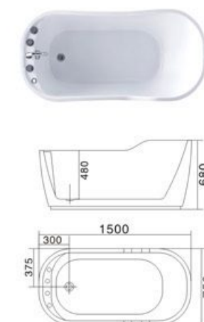
Model: H-8019 SIZE: 1500x750x680mm
