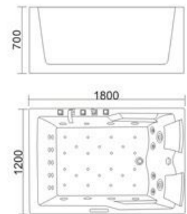
Model: H-002A SIZE: 1800x1200x700mm 左右裙 Left/Right Skirt
