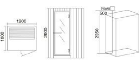
LN-1019 铁杉木 Hemlock 1200x1000x2000mm 非标订造 Non-standard manufactured 可做桑拿房、光波房、频谱房 Saund Room、Far-Infrsred Steam Room、 Spectrum Room
