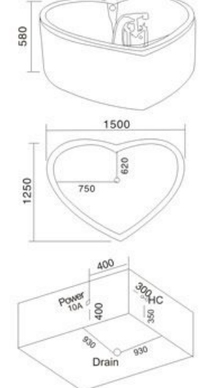
Model: H-1513 SIZE: 1500x1250x580mm
