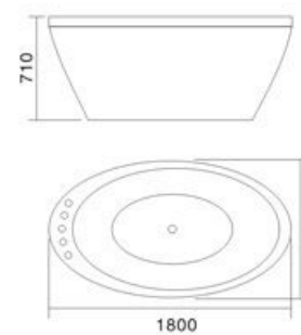
Model: H-005 SIZE: 1800x900x710mm
