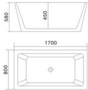
Model: H-7012A SIZE: 1500x750x580mm 1600x800x580mm 1700x800x580mm
