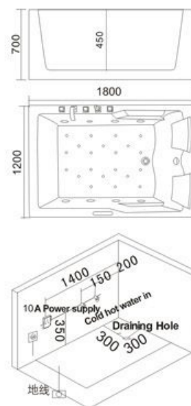
Model: H-002 SIZE: 1800x1200x700mm 1700x1200x700mm 左右裙 Left/Right Skirt
