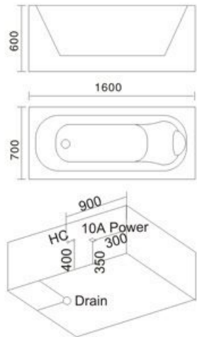
Model: H-081 SIZE: 1600x700x600mm 左右裙 Left/Right Skirt
