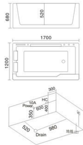
Model: H-008 SIZE: 1700x1200x680mm
