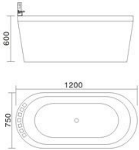
Model: H-06 SIZE: 1200x750x600mm 1300x750x600mm 1400x750x600mm 1500x750x600mm
