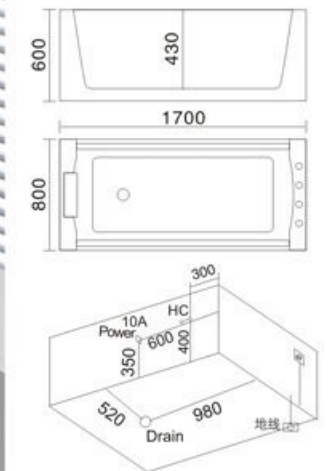
Model: H-1701 SIZE: 1700x800x600mm
