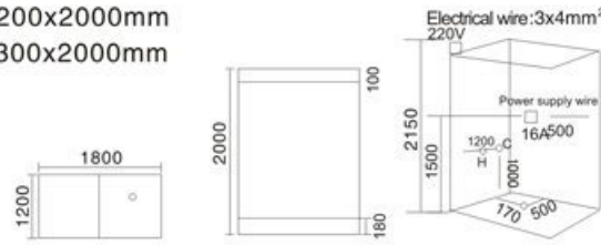
Model: LN-1613 SIZE: 1800x1200x2000mm 2000x1300x2000mm
