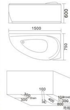
Model: H-067 SIZE: 1400x750x600mm 1500x750x600mm 1600x750x600mm 1700x750x600mm
