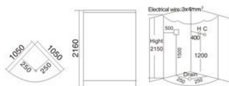
Model: A-004 SIZE: 1050x1050x2160mm
