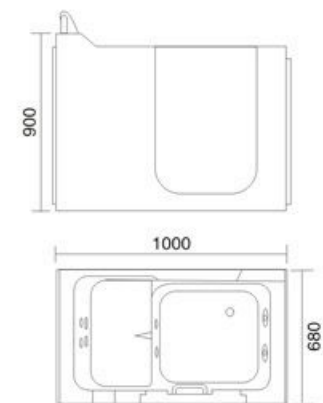
Model: H-5620 SIZE: 1000x680x900mm
