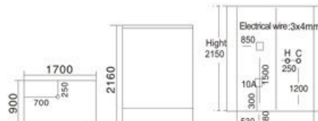
Model: AB-024 SIZE: 1700x900x2160mm
