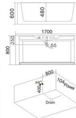
Model: H-1700 SIZE: 1700x800x600mm
