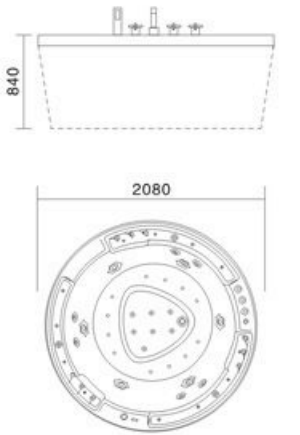
Model: H-5611 SIZE: 2080x2080x840mm
