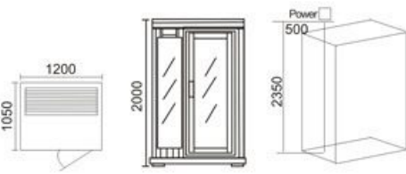
LN-1029 铁杉木 Hemlock 1200x1050x2000mm 非标订造 Non-standard manufactured 可做桑拿房、光波房、频谱房 Saund Room、Far-Infrsred Steam Room、 Spectrum Room
