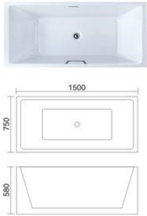
Model: H-8011 SIZE: 1500x700x580mm 1500x750x580mm 1600x750x580mm 1700x750x580mm
