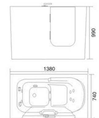
Model: H-5625 SIZE: 1380x740x990mm 左右裙 Left/Right Skirt
