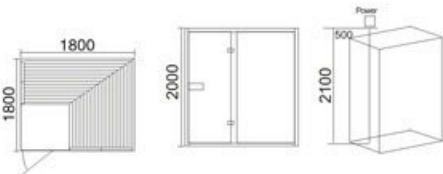
LN-1049 铁杉木 Hemlock 1800x1800x2000mm 非标订造 Non-standard manufactured 可做桑拿房、光波房、频谱房 Saund Room、Far-Infrsred Steam Room、 Spectrum Room
