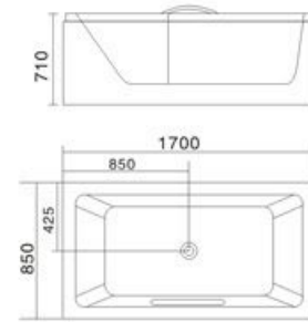
Model: H-001 SIZE: 1700x850x710mm
