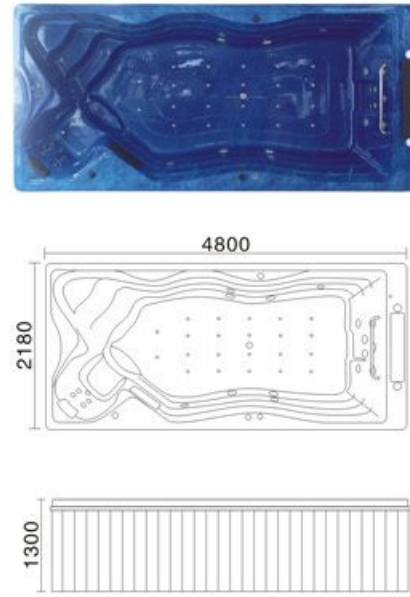
Model: H-5506 SIZE: 4800x2180x1300mm
