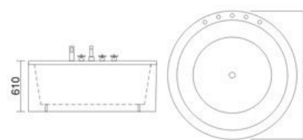
Model: H-03 SIZE: 1000x1000x610mm 1200x1200x610mm 1300x1300x610mm 1500x1500x610mm 1600x1600x610mm 1700x1700x610mm 1800x1800x610mm 1900x1900x610mm 2000x2000x610mm
