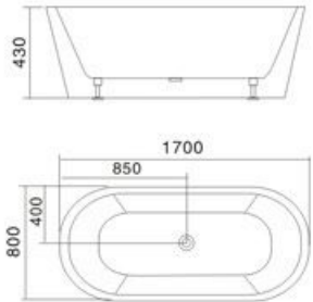
Model: H-7003B SIZE: 1200x650x430mm 1300x700x430mm 1400x700x430mm 1500x750x430mm 1600x750x430mm 1600x800x430mm 1700x750x430mm 1700x800x430mm
