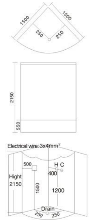
Model: A-092 SIZE: 1500x1500x2150mm
