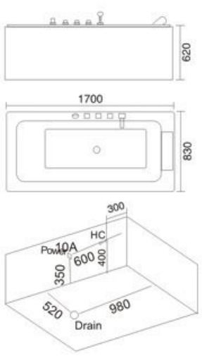
Model: H-1783 SIZE: 1700x830x620mm 左右裙 Left/Right Skirt
