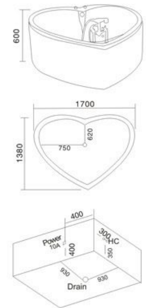
Model: H-1713 SIZE: 1700x1380x600mm
