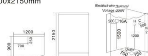
Model: A-120 SIZE: 1200x900x2150mm
