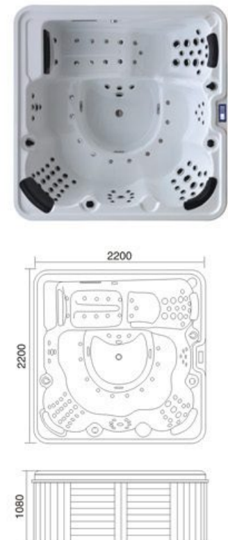
Model: H-5312 SIZE: 2200x2200x1080mm
