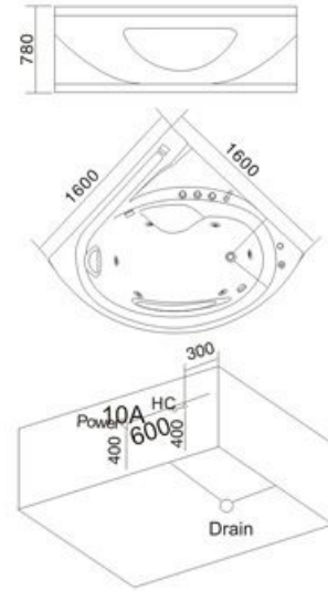
Model: H-1681 SIZE: 1600x1600x780mm
